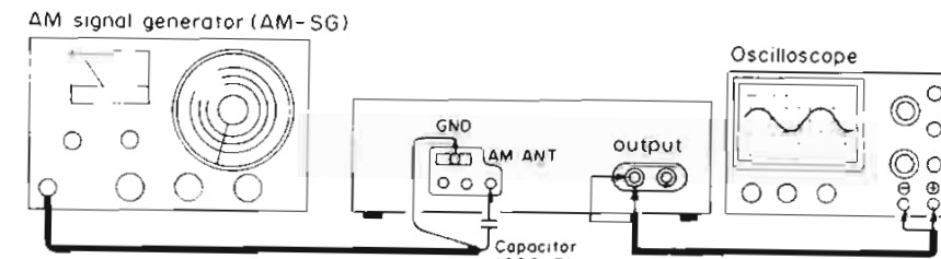
[Fig. 3] AM adjustment
