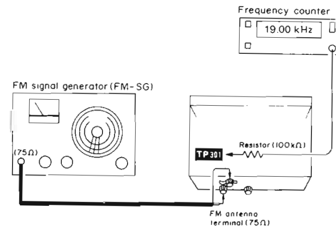
[Fig. 6] FM MPX VCO adjustment
