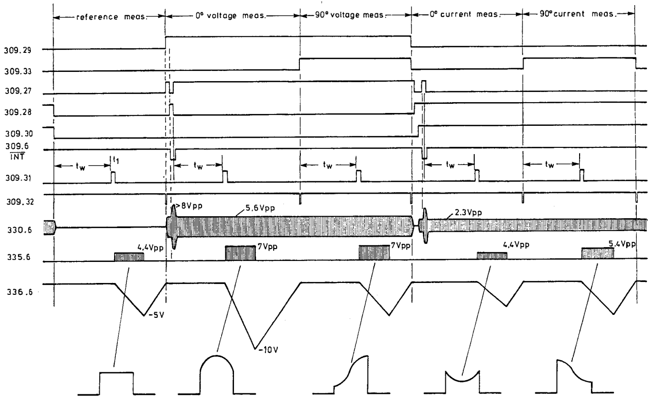
Fig. 7 One complete measurement cycle (CUT = 100 k \Omega )
