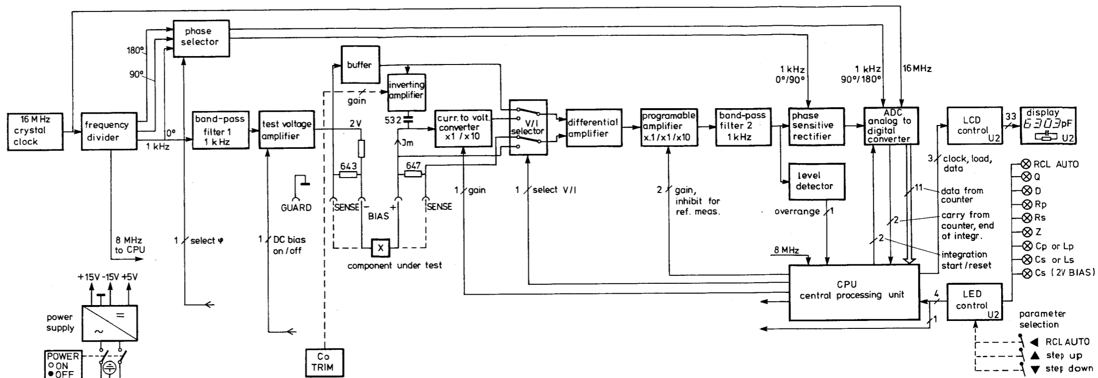
Fig. 3 Block diagram
