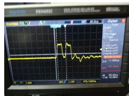
TDR scope time delay measurement
