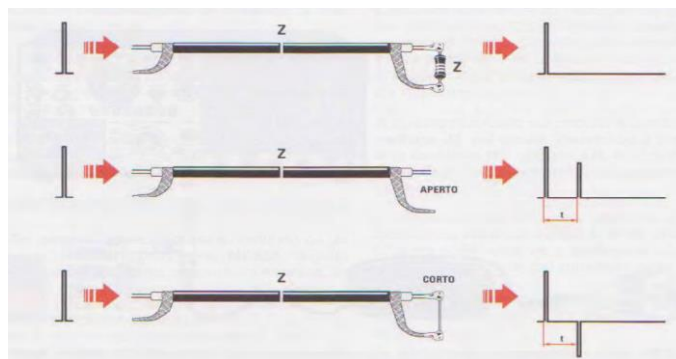
TDR Coaxial cable Pulse shape
