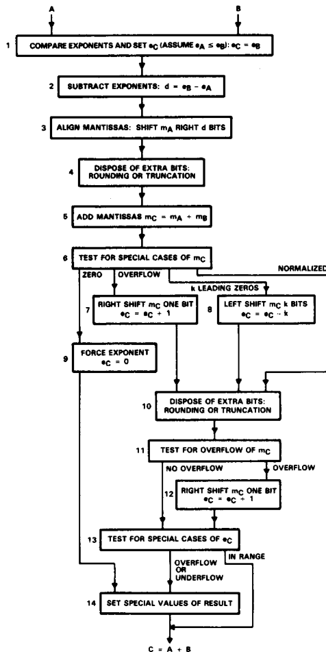
Figure 2. Floating-Point Addition
